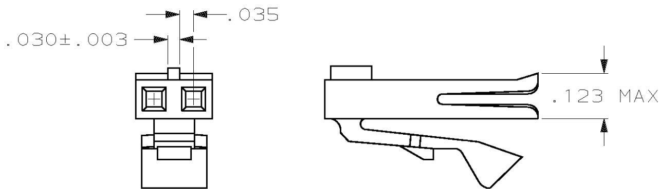
DETAIL FOR 2 POSN ONLY
