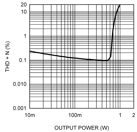
THD+N vs Output Power 3V, 4 \Omega , BTL at 1kHz
