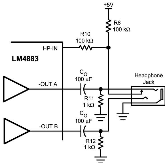
FIGURE 4. Headphone Circuit
