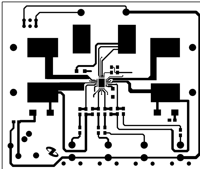
FIGURE 5. Top Layer
