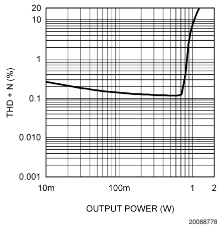
THD+N vs Output Power 3V, 8 \Omega , SE at 1kHz
