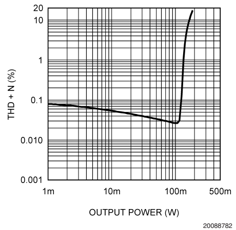
THD+N vs Output Power 3V, 32 \Omega , SE at 1kHz
