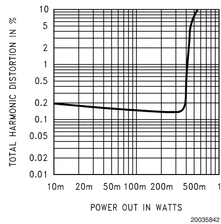
THD+N vs Power Out at V_{DD} = 3.3V , 8\Omega R_L , 1kHz
