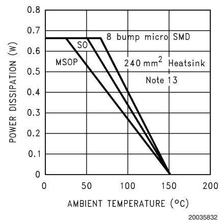
Power Derating Curves (P DMAX = 670mW)
