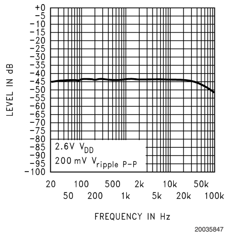
Power Supply Rejection Ratio (PSRR) at V_{DD} = 2.6V
