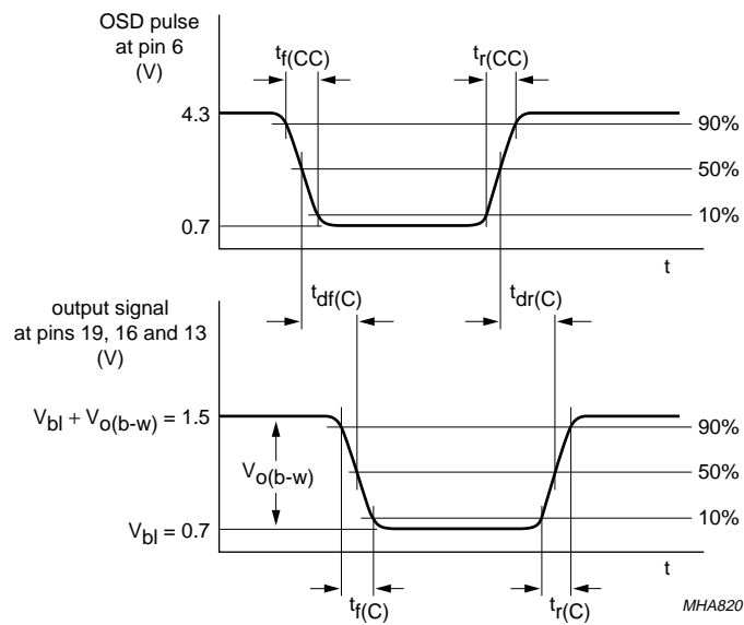
Fig.10 Typical OSD fast blanking input/output waveforms.
