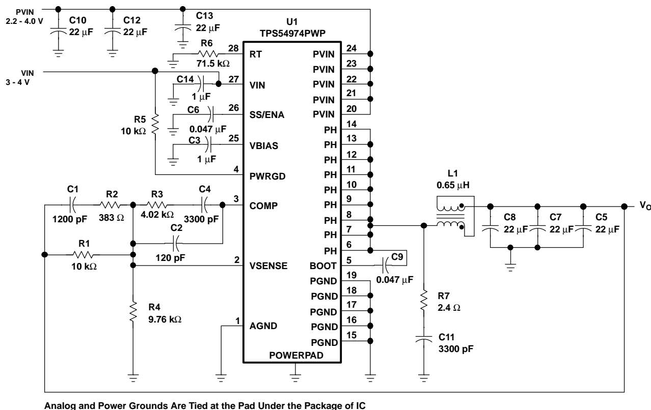
Figure 10. Application Circuit
