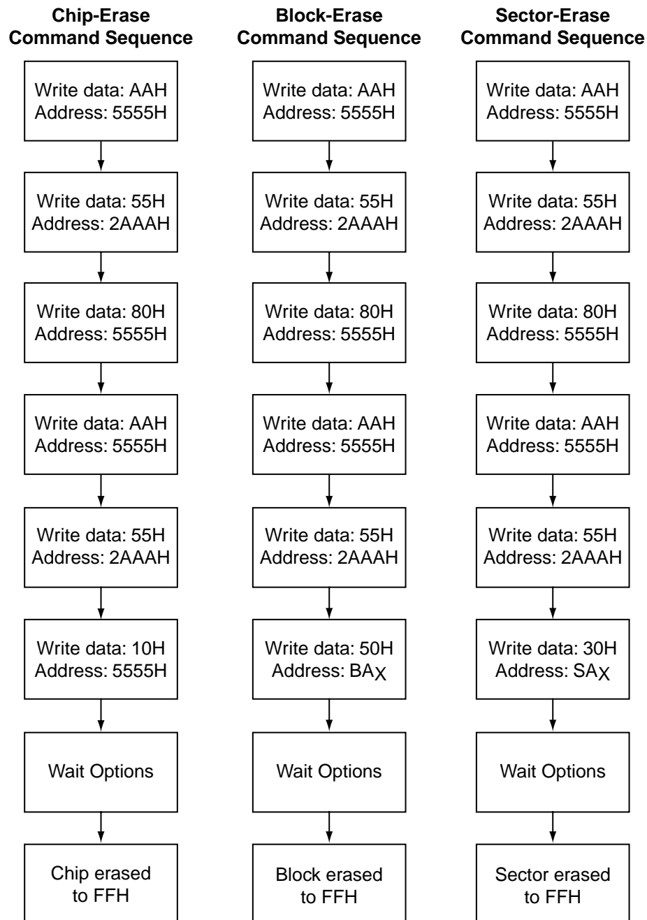
FIGURE 29: ERASE COMMAND SEQUENCE
