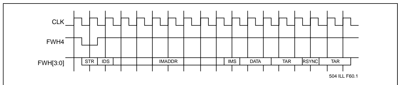
FIGURE 2: WRITE WAVEFORMS
