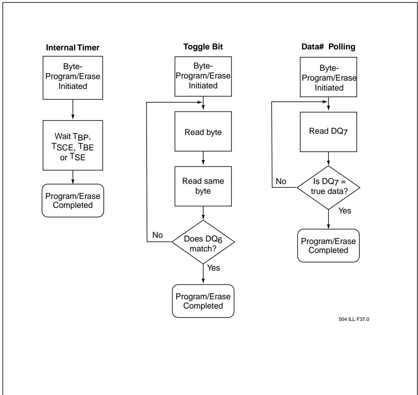
FIGURE 27: WAIT OPTIONS
