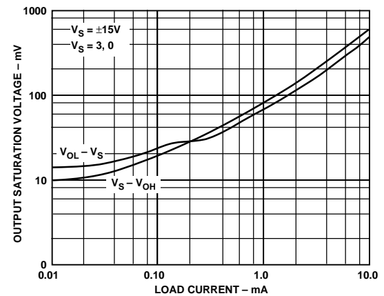
Figure 28. Output Saturation Voltage
