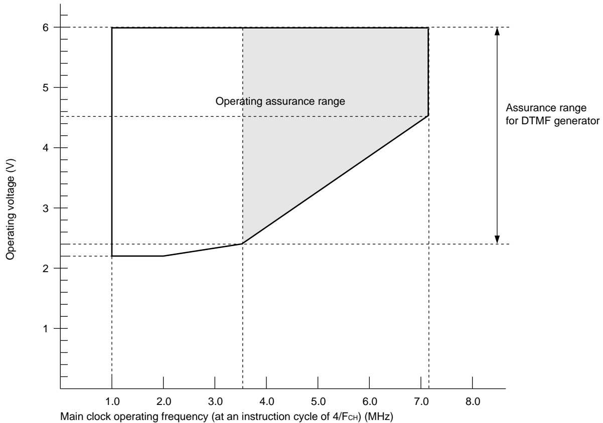
Figure 1 Operating Voltage vs. Main Clock Operating Frequency(MB89170/170A series)
