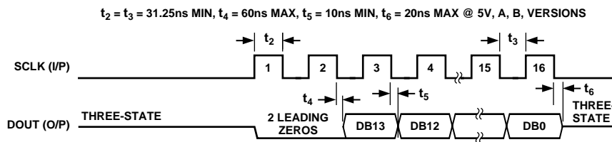
Figure 5. Data Read Operation
