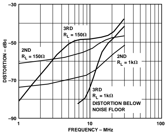
Figure 15. Distortion vs. Frequency; V_S = \pm 5V , G = +2
