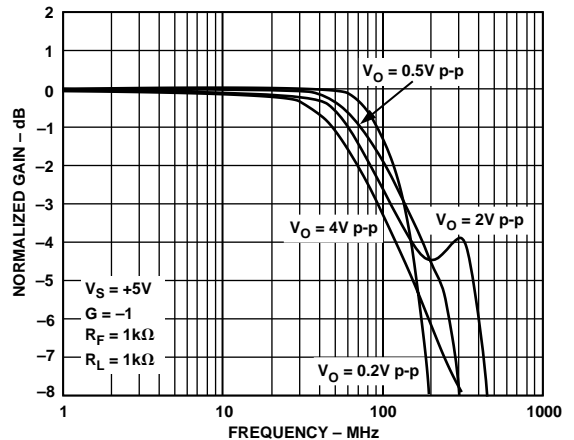
Figure 6. Bandwidth vs. Output Level—Single Supply, Gain of -1
