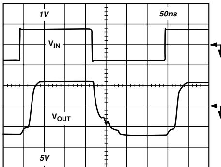
Figure 33. 15% Overload Recovery, Gain = 10 ( R_{FB} = 400 \Omega , R_L = 1 k\Omega , V_S = \pm 7.5 V )
