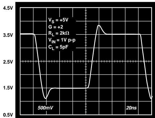
Figure 29. One Volt Step Response, V_S = +5\text{ V} , G = +2
