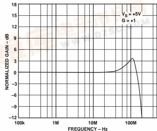
Figure 2. Frequency Response: Gain = +1, V S = +5 V
