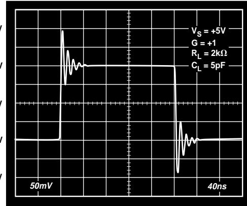
Figure 30. 100 mV Step Response, V_S = +5\text{ V} , G = +1
