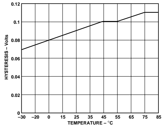
Figure 5. Hysteresis vs. Temperature for SU3—Low to High
