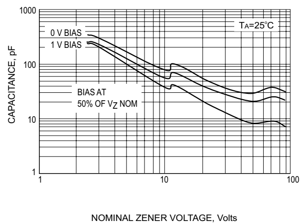
TYPICAL CAPACITANCE
