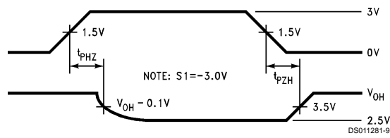
FIGURE 6. Receiver TRI-STATE Timing ( t_{PHZ} , t_{PZH} )
