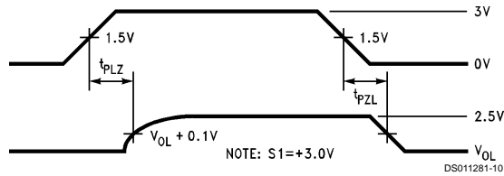
FIGURE 7. Receiver TRI-STATE Timing ( t_{PLZ} , t_{PZL} )
