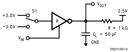
FIGURE 5. Receiver Disable Load Circuit
