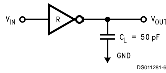
FIGURE 3. Receiver Load Circuit
