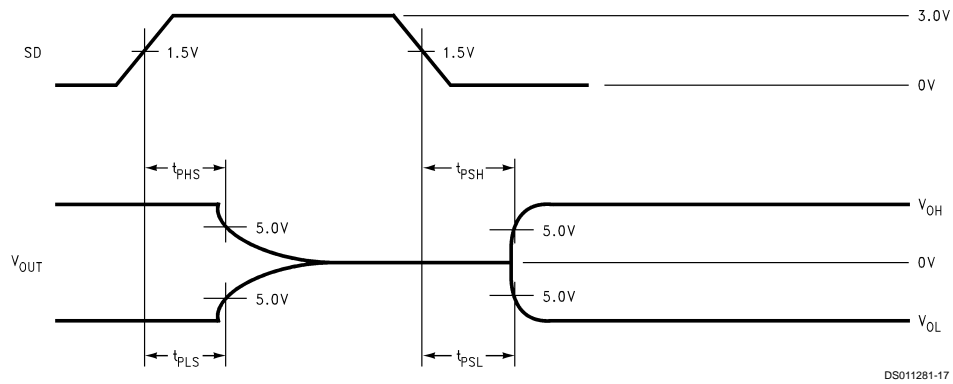
FIGURE 9. Driver Shutdown (SD) Delay Timing Waveforms
