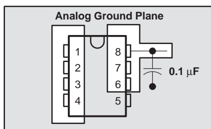
Figure 16. Power-Supply Bypassing
