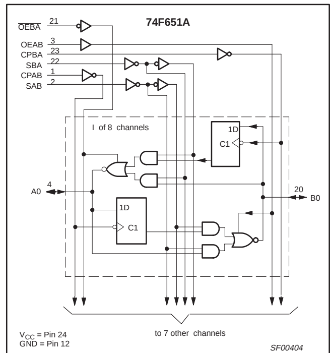
LOGIC DIAGRAM
