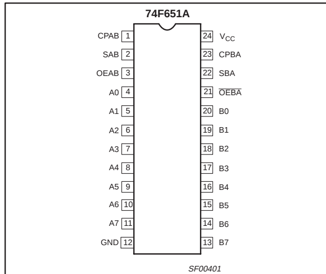
PIN CONFIGURATION
