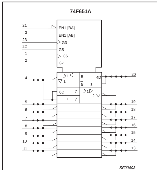
IEC/IEEE SYMBOL
