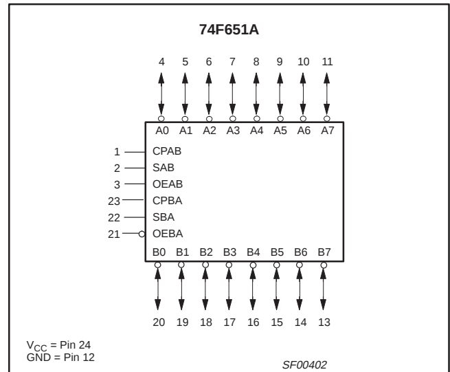
LOGIC SYMBOL
