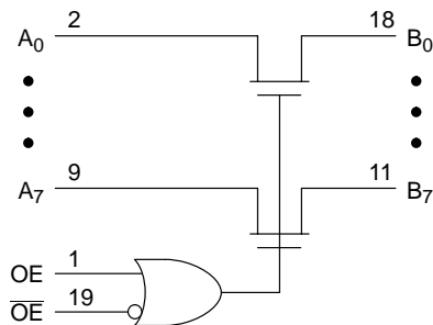
Figure 2. Logic Diagram
