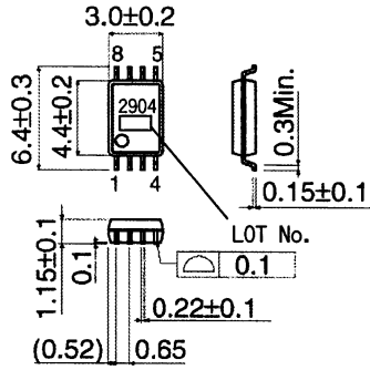
BA2904FV(SSOP-B8) (Unit: [mm])
