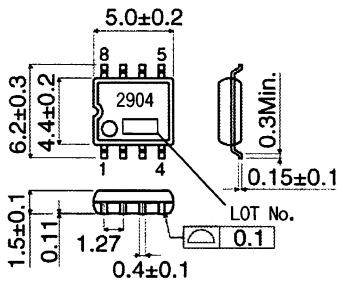
BA2904F(SOP8) (Unit: [mm])
