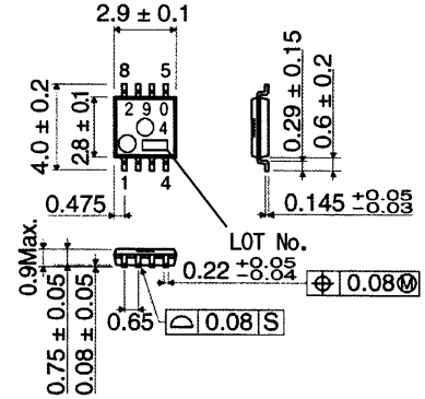
BA2904FVM(MSOP8) (Unit: [mm])
