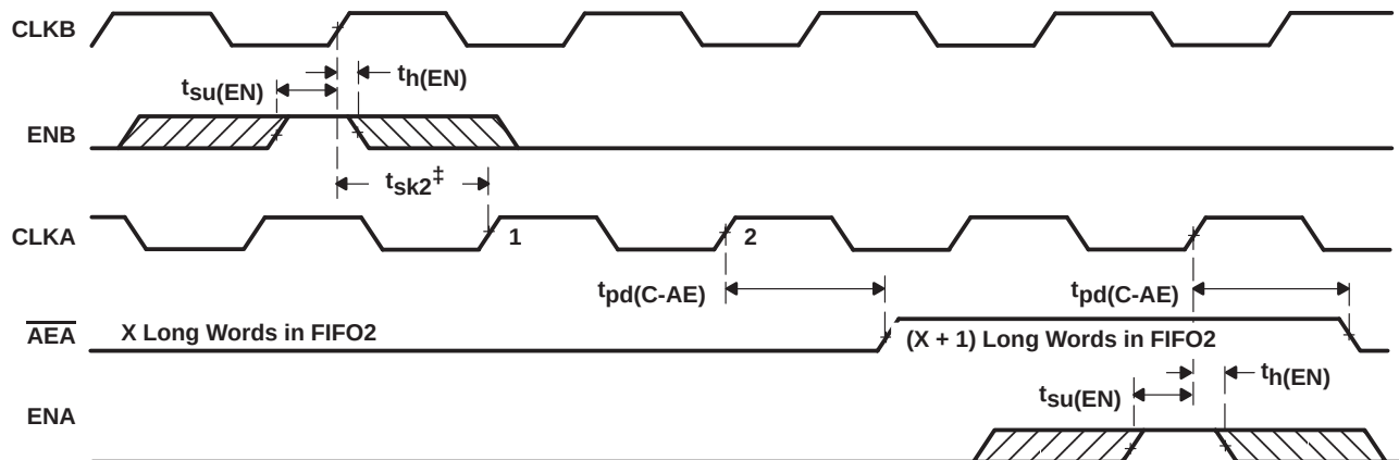
Figure 17. \overline{AEB} When FIFO1 Is Almost Empty
