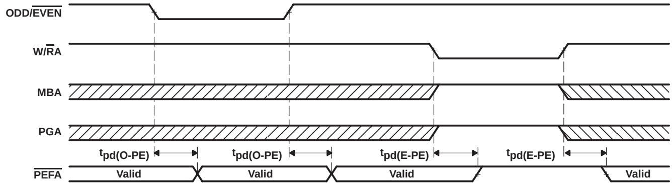
Figure 23. ODD/EVEN, W/RA, MBA, and PGA to PEFA
