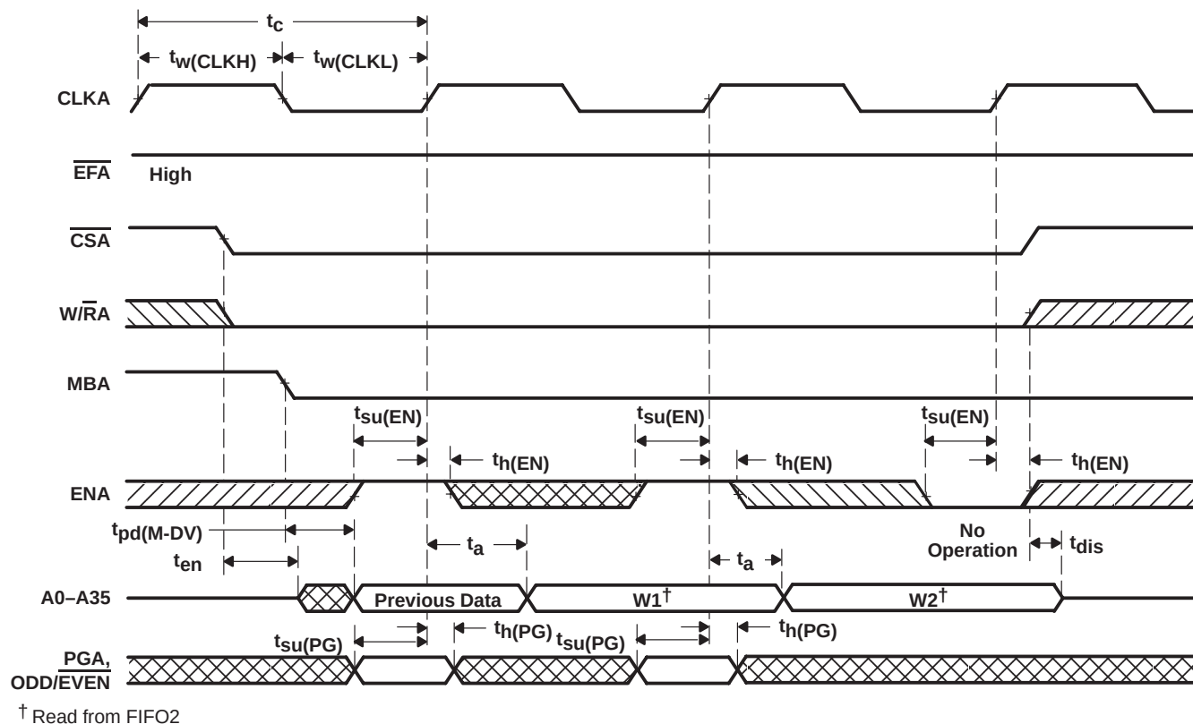
Figure 12. Port-A Read Cycle for FIFO2
