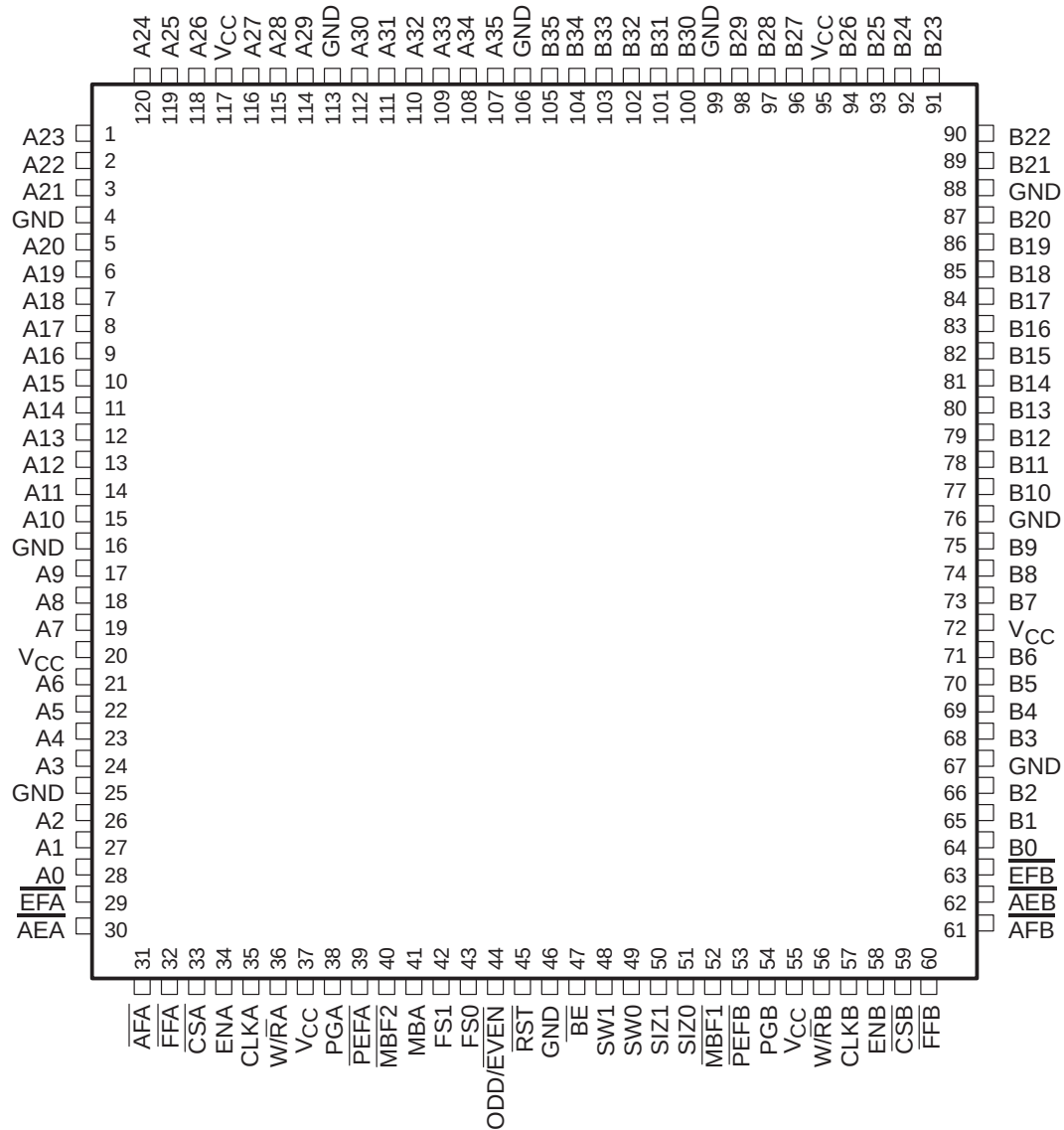
PCB PACKAGE (TOP VIEW)
