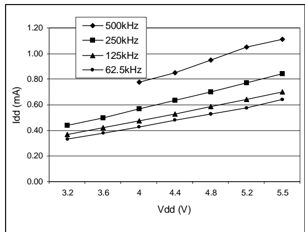
Figure 64. Typical I_{DD} in SLOW vs. f_{CPU}
