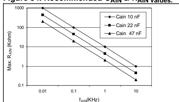
Figure 94. Recommended C_{AIN} & R_{AIN} values. 5)
