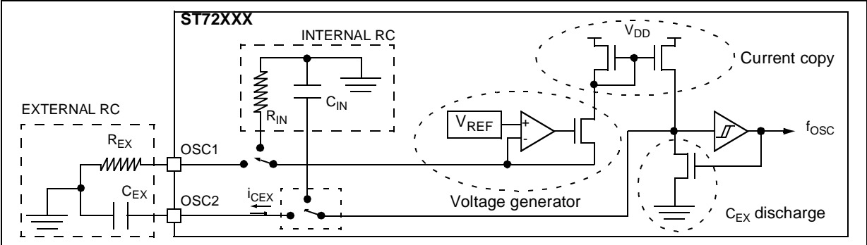
Figure 69. Typical Application with RC oscillator
