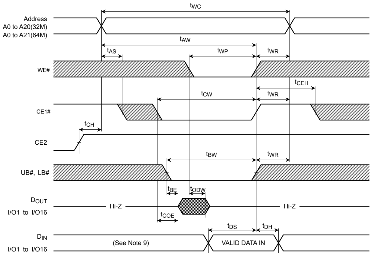
Figure 53. Write Cycle #2 (CE# Controlled) (See Note 8)
