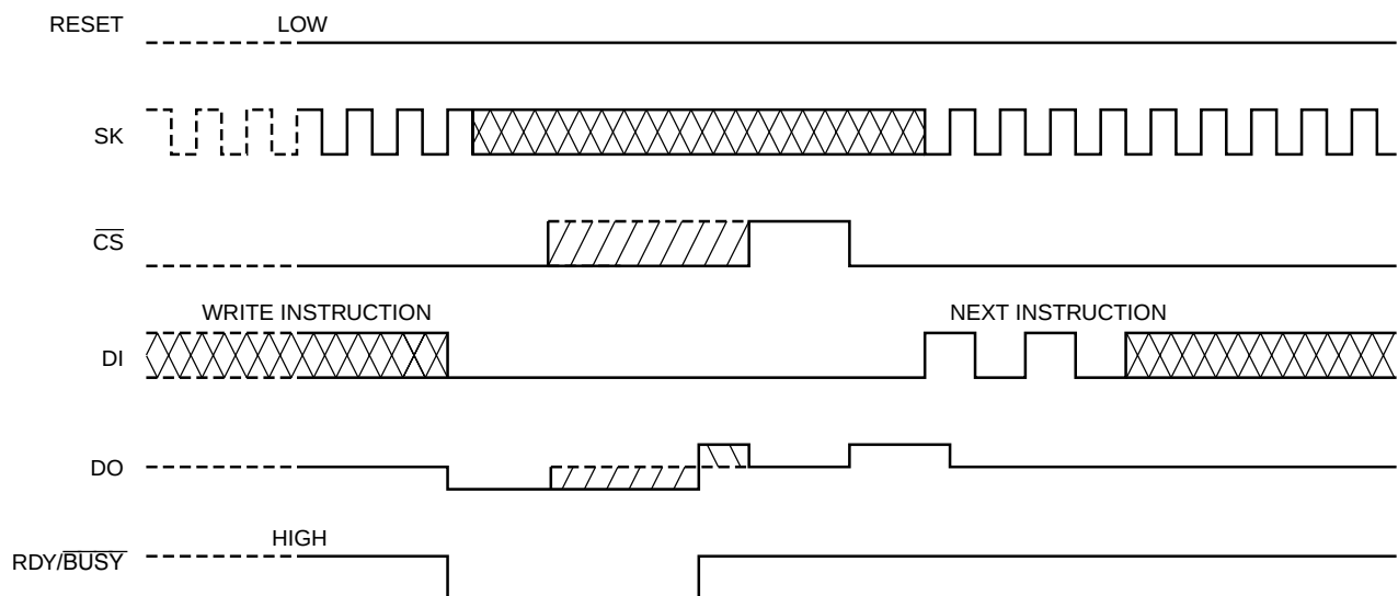
Figure 5. Ready/ \overline{BUSY} Status Instruction Timing
