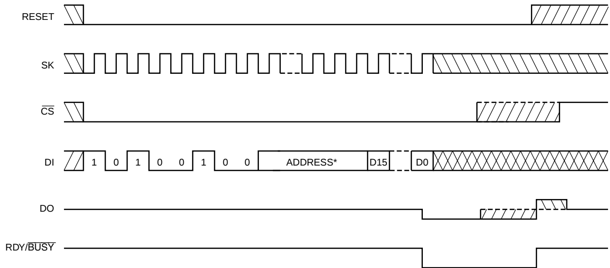
Figure 4. Write Instruction Timing
