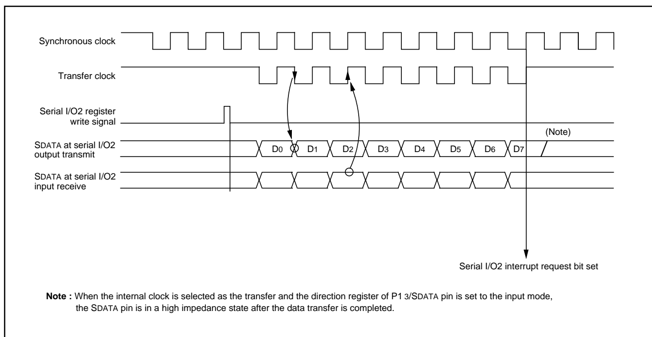
Fig. 34 Serial I/O2 timing (LSB first)
