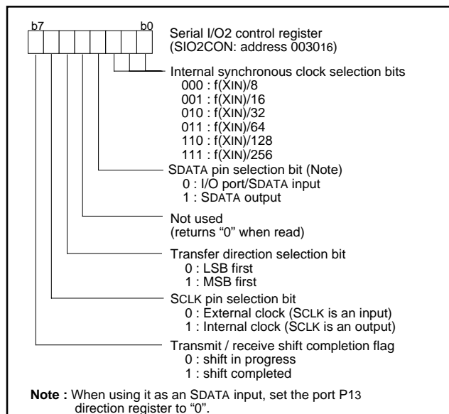
Fig. 32 Structure of serial I/O2 control registers
