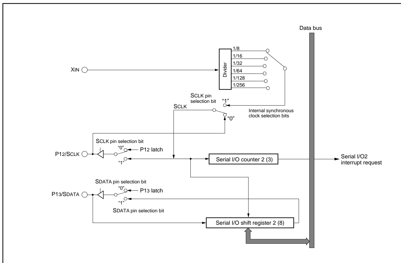
Fig. 33 Block diagram of serial I/O2
