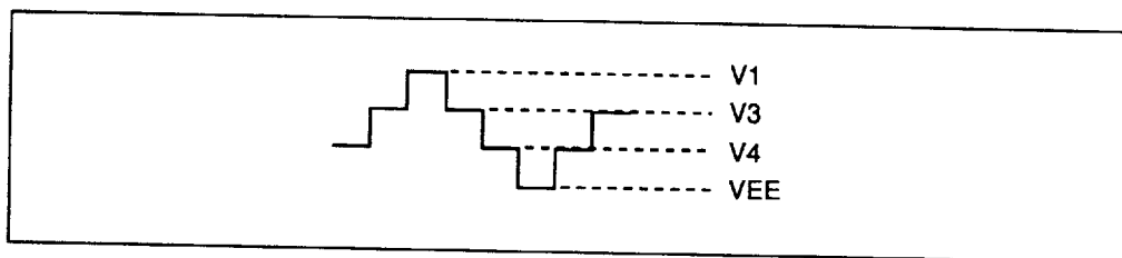
Figure 1 Different Power Supply Voltage Levels for LCD Drive Circuits
