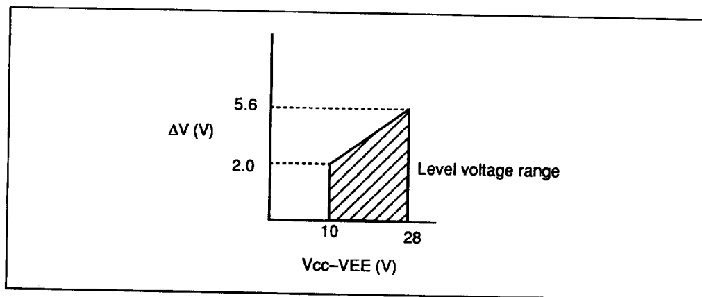
Figure 7 Relation between V_{CC} - V_{EE} and \Delta V
