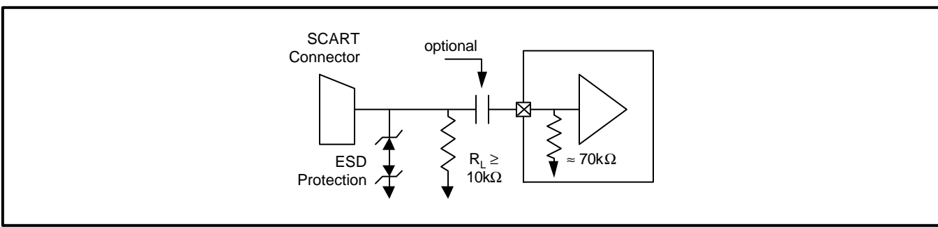
Audio Input Circuit
