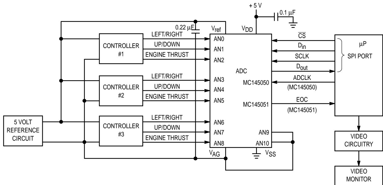
Figure 15. Joystick Interface
