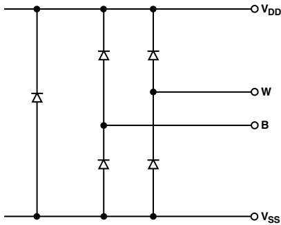
Figure 7. Maximum Terminal Voltages Set by V_{DD} and V_{SS}
