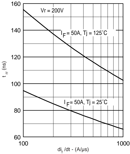
Fig. 6 - Typical Reverse Recovery vs. di_t/dt
