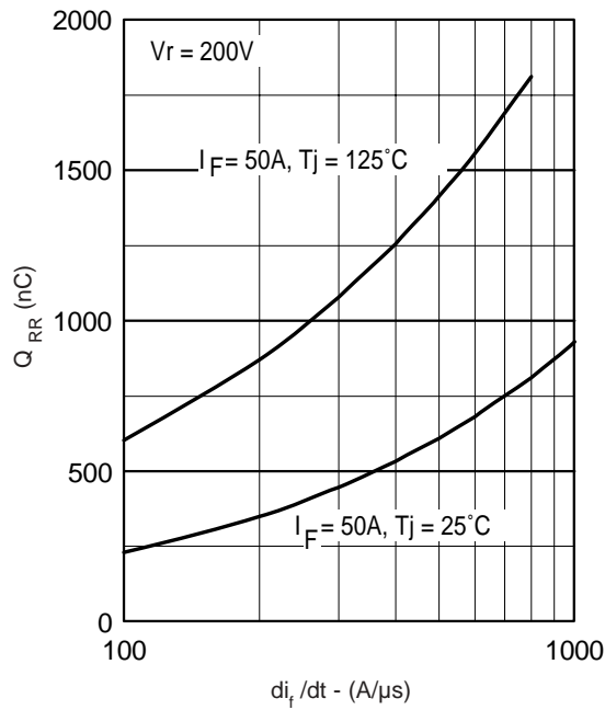
Fig. 8 - Typical Stored Charge vs. di_t/dt
