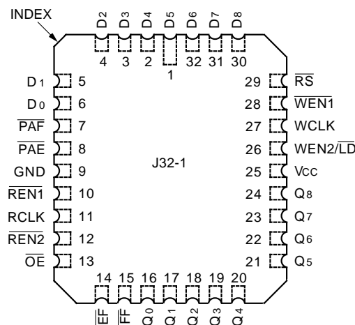
PLCC TOP VIEW
