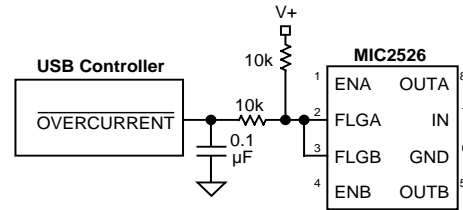
Figure 4. Transient Filter
