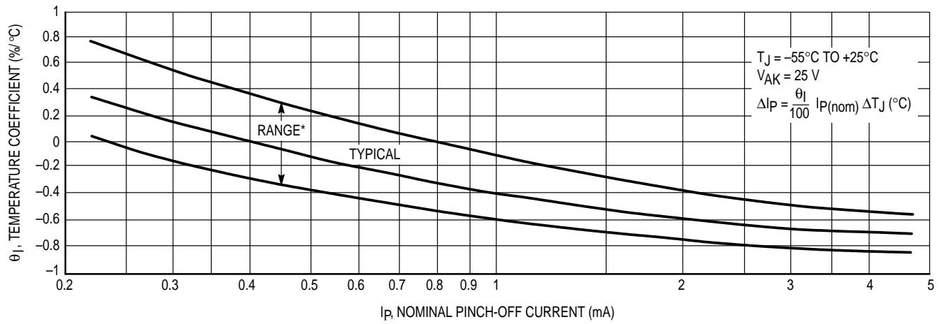
Figure 5. Temperature Coefficient
