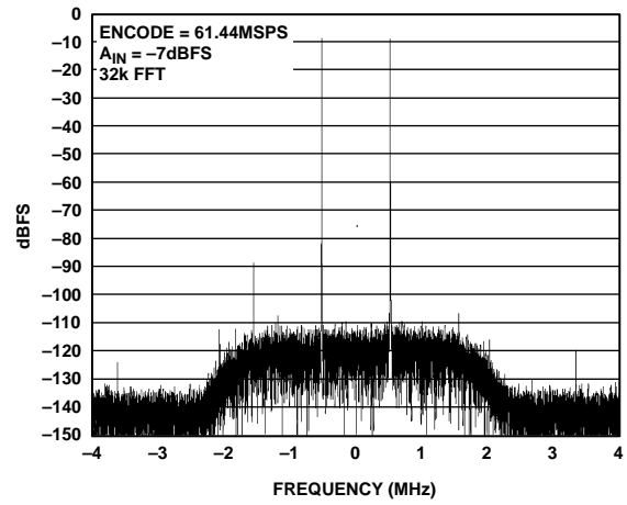
Figure 11. Two Tones at 55 MHz and 56 MHz
