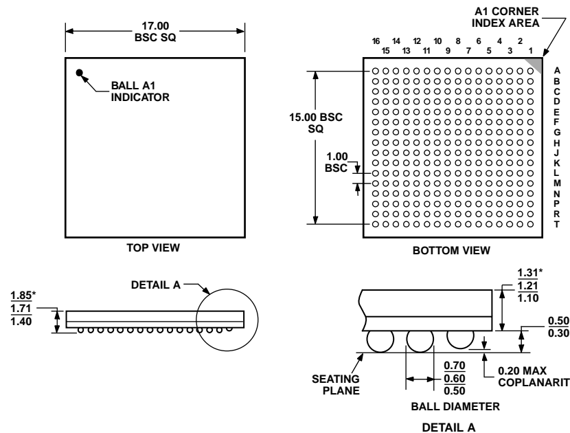
Figure 66. 256-Lead Chip Scale Ball Grid Array [CSPBGA] (BC-256-2) Dimensions shown in millimeters
