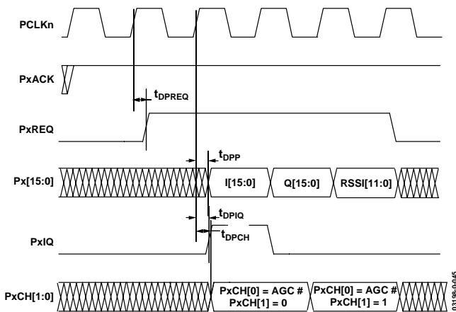
Figure 58. AGC with RSSI Word
