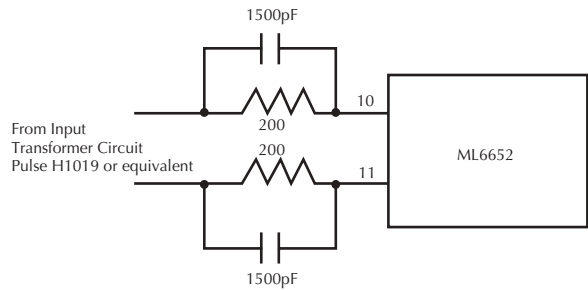
Figure 1. Twisted Pair Interface Mode Input Networks
