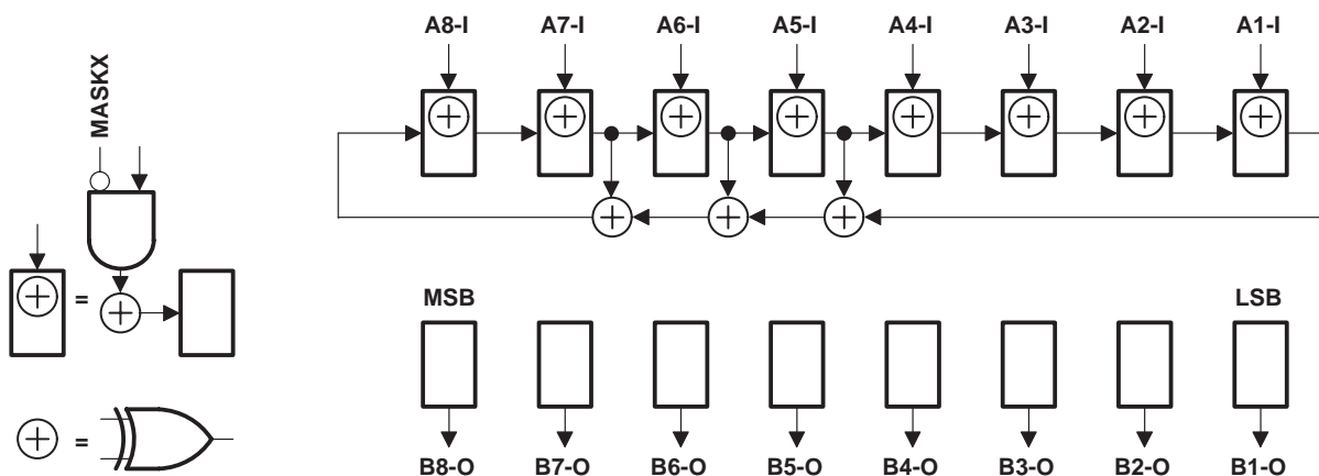
Figure 11. 8-Bit PSA/COUNT Configuration ( OEAB = 1 , \overline{OEBA} = 1 )
