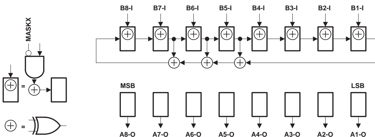
Figure 12. 8-Bit PSA/COUNT Configuration ( OEAB = 0 , \overline{OEBA} = 0 )
