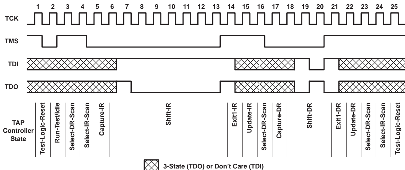
Figure 13. Timing Example
