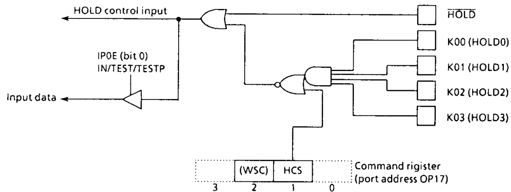
Figure 4-1. Hold control circuit
