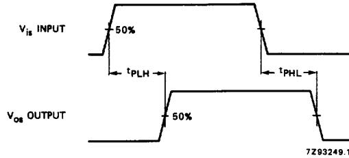
Fig.18 Waveforms showing the input ( V_{is} ) to output ( V_{0s} ) propagation delays.
