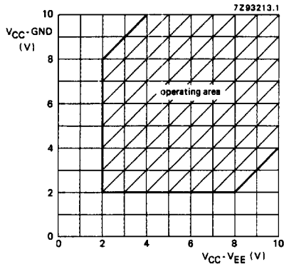
Fig.6 Guaranteed operating area as a function of the supply voltages for 74HC4053.
