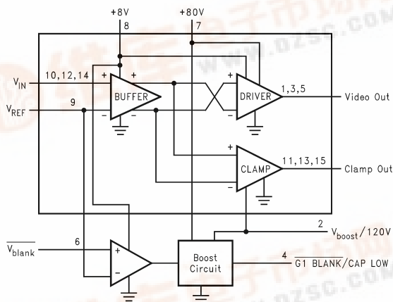
FIGURE 1. LM2453 Block Diagram
