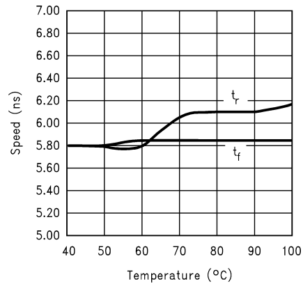
FIGURE 6. CRT Driver Speed vs. Temperature
