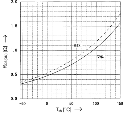
Drain-Source On-State Resistance vs. T_{ch} R_{DS(on)} = f(T_{ch}) ; I_D=5\text{A} ; V_{GS}=10\text{V}
