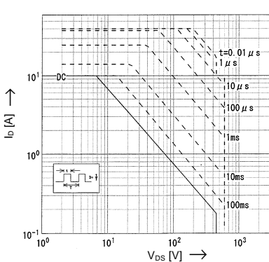
Safe Operation Area I_D = f(V_{DS}) ; D=0,01 ; T_{ch}=25^\circ\text{C}
