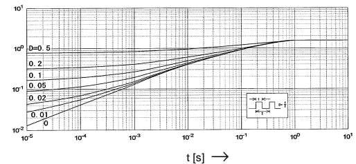
Transient Thermal Impedance Z_{th(jc)} = f(t) parameter: D=t/T
