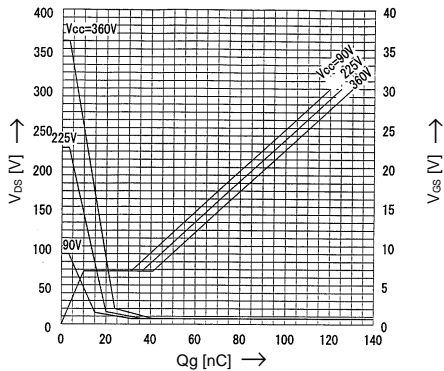
Typical Gate Charge Characteristic V_{GS} = f(Q_g) ; I_D=10\text{A} ; T_{ch}=25^\circ\text{C}
