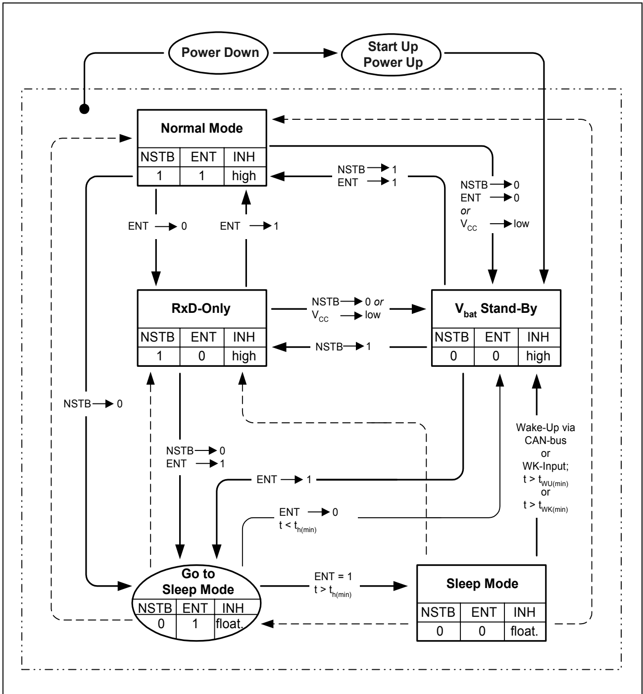
Figure 4 State Diagram
