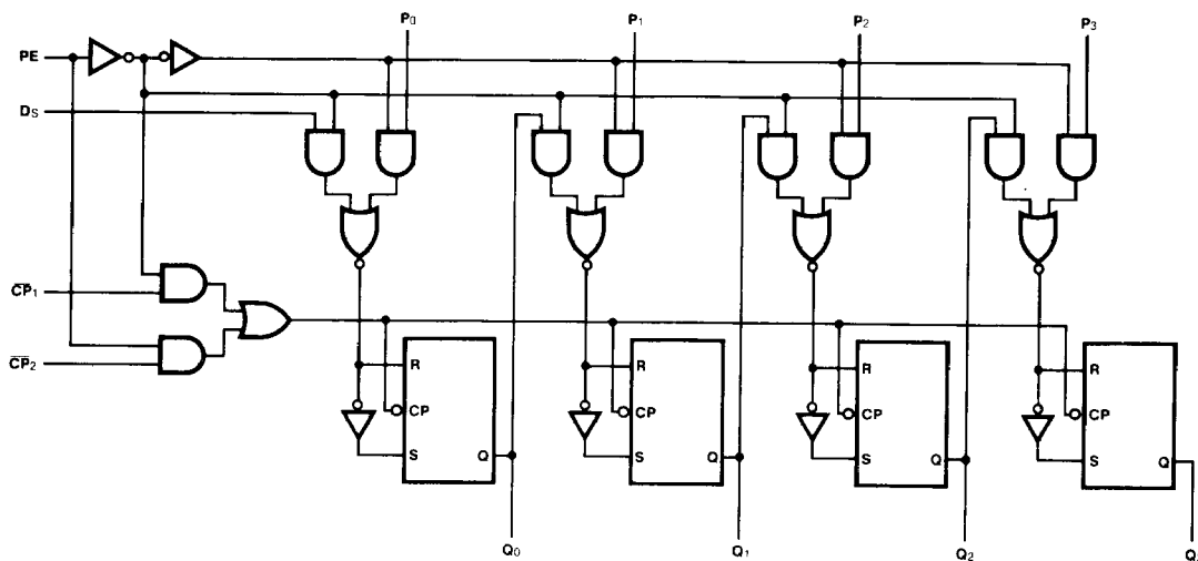
LOGIC DIAGRAM
