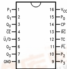
Pin Assignment for DIP and Flatpack
