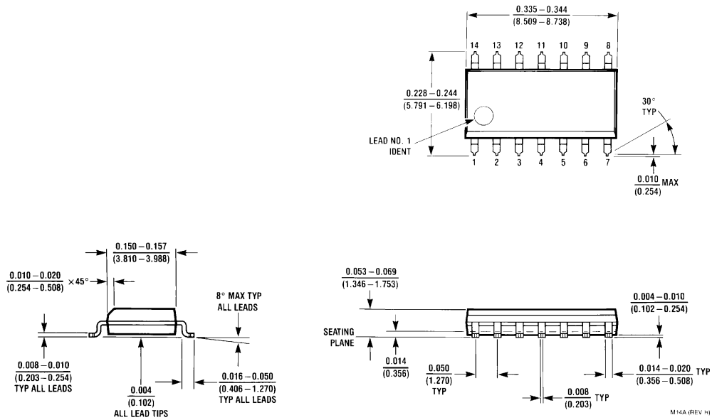
14-Lead Small Outline Molded Package (M) Order Number DM74LS02M NS Package Number M14A
