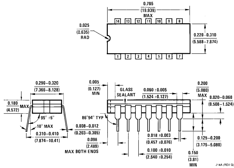
14-Lead Ceramic Dual-In-Line Package (J) Order Number 54LS02DMQB or DM54LS02J NS Package Number J14A
