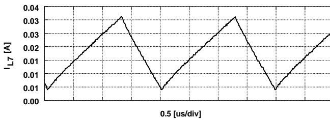
CH-7 Peak Current Waveform (MODE7 = L, Input: VCH3, Output: 150 mA)
