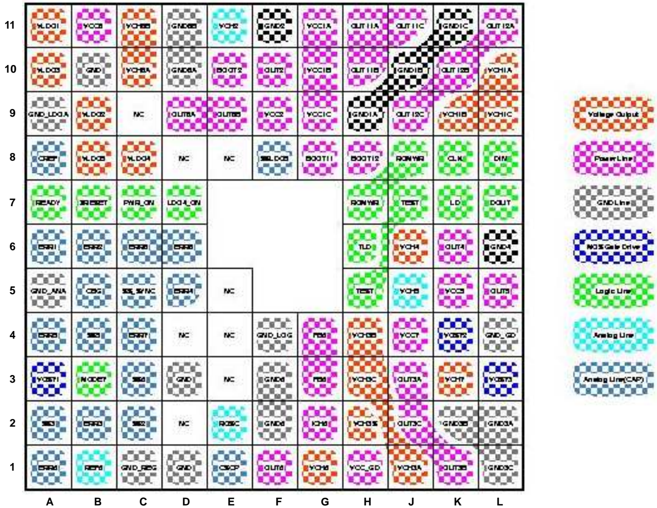
Figure 15. Pin Layout
