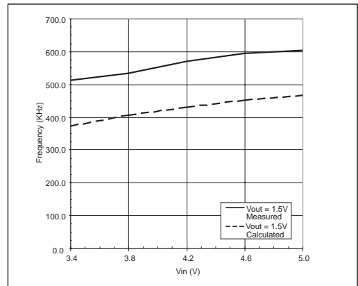
Ripple Frequency vs. V_{IN} , I_{OUT} = 0.4A , V_{OUT} = 1.5V
