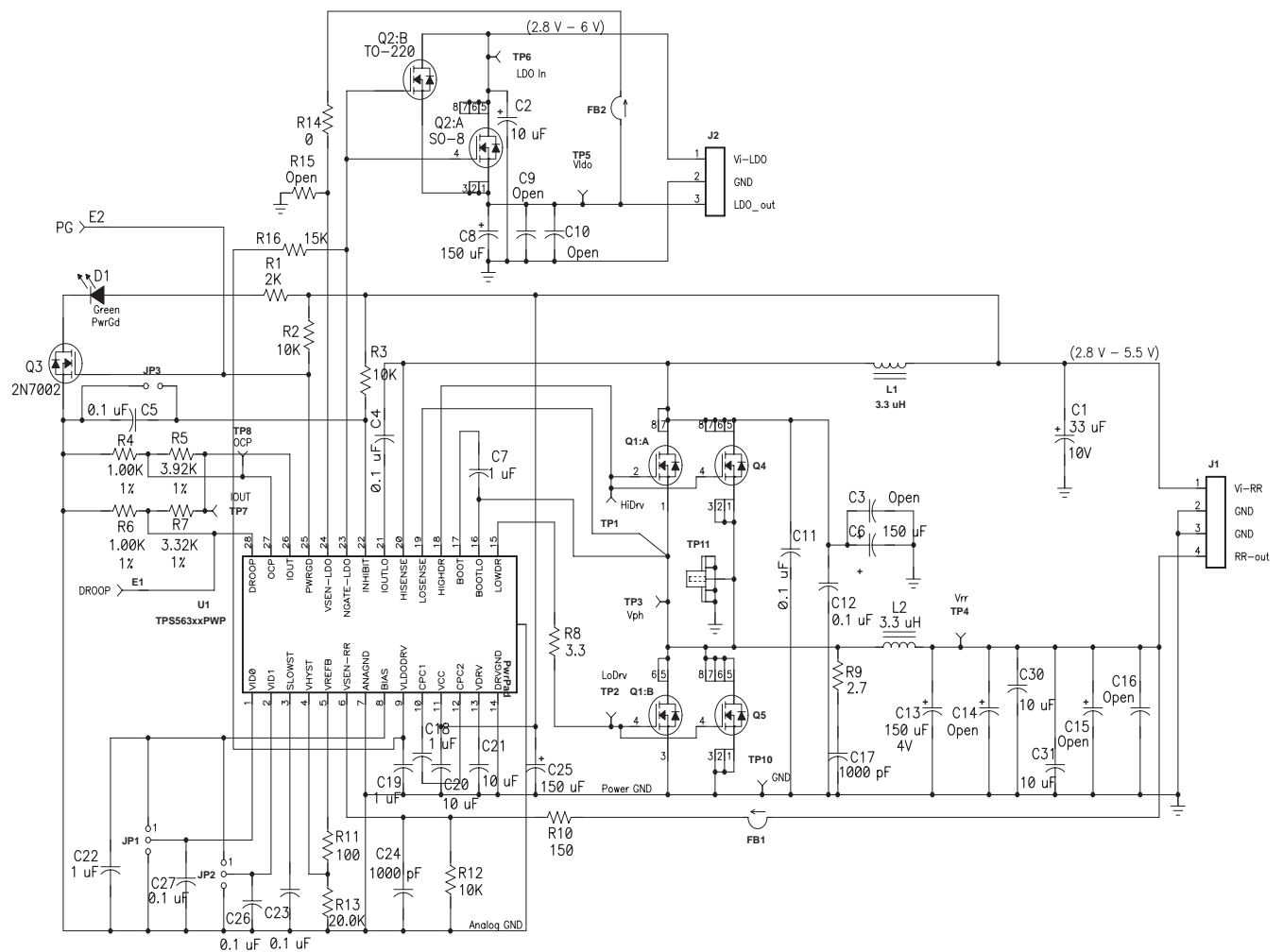
Figure 22. EVM Schematic
