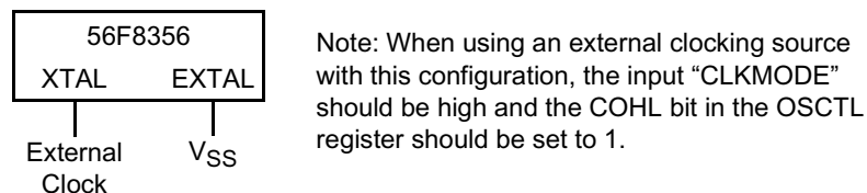
Figure 3-4 Connecting an External Clock Register
