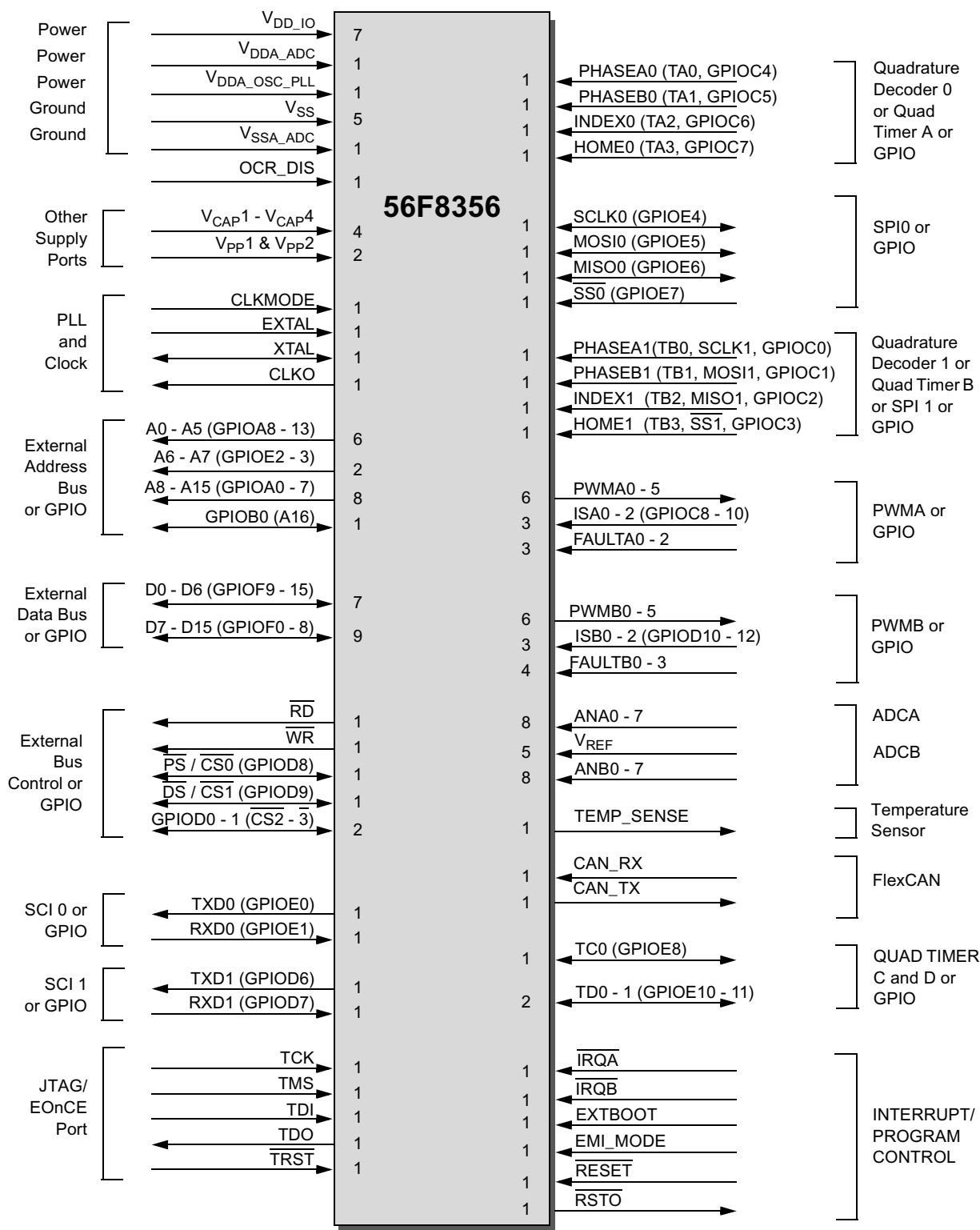
Figure 2-1 56F8356 Signals Identified by Functional Group 1 (144-pin LQFP)
