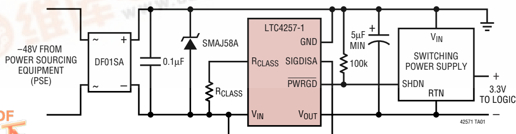
Powered Device (PD)
