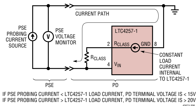
Figure 5. IEEE 802.af Measured-Voltage Method of Classification Probing
