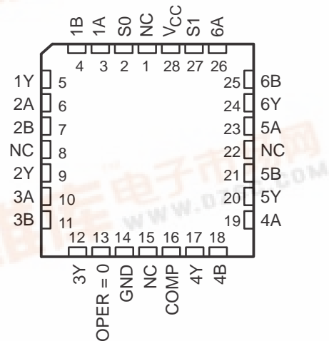
SN54ALS857 ... FK PACKAGE (TOP VIEW)
