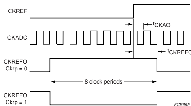
Fig 8. Timing diagram; CKREFO; Dmx = 0.
