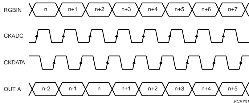
Fig 11. Timing diagram; single port mode; Dmx = 0, Ckdd = 0, Ckdp = 0; n = even pixel.
