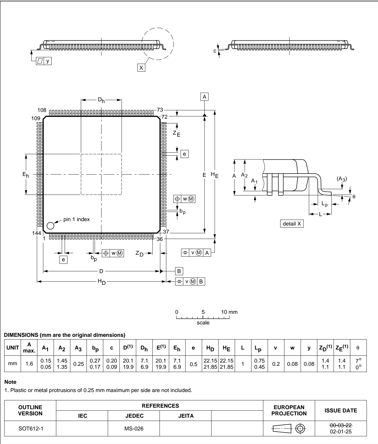
Fig 17. Package outline.
